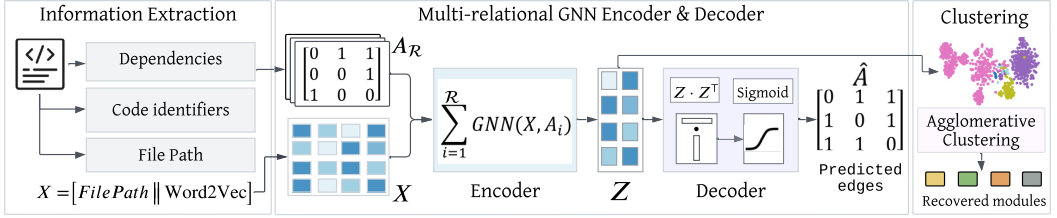
Fig. 1. Overview of the GAER pipeline. Source code is transformed into a multi-relational dependency graph with node features derived from Word2Vec-embedded code identifiers and binary directory-path vectors. A multi-relational heterogeneous GNN encoder learns node embeddings Z within the GAE framework, which are clustered to recover architectural modules.
