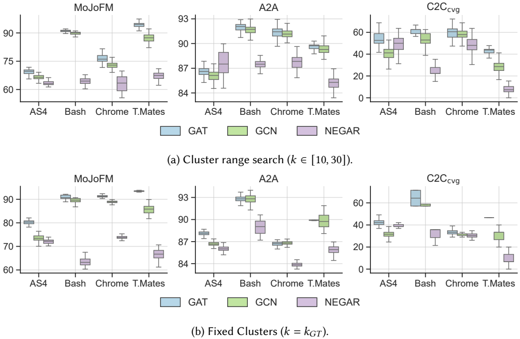
Fig. 2. Run-to-run variability over 100 seeds on four representative systems. Top: k selected via range search. Bottom: k fixed to the reference module count.
